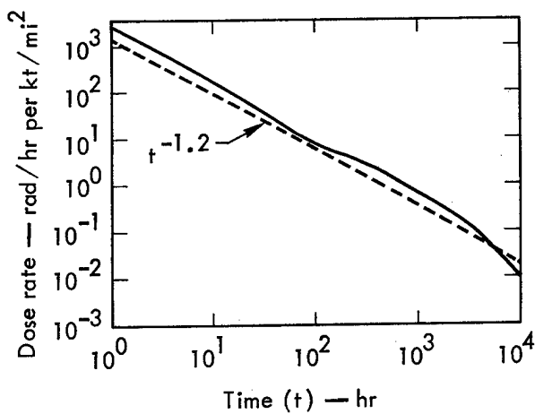
Fig. A-3. Fission-product delay.
